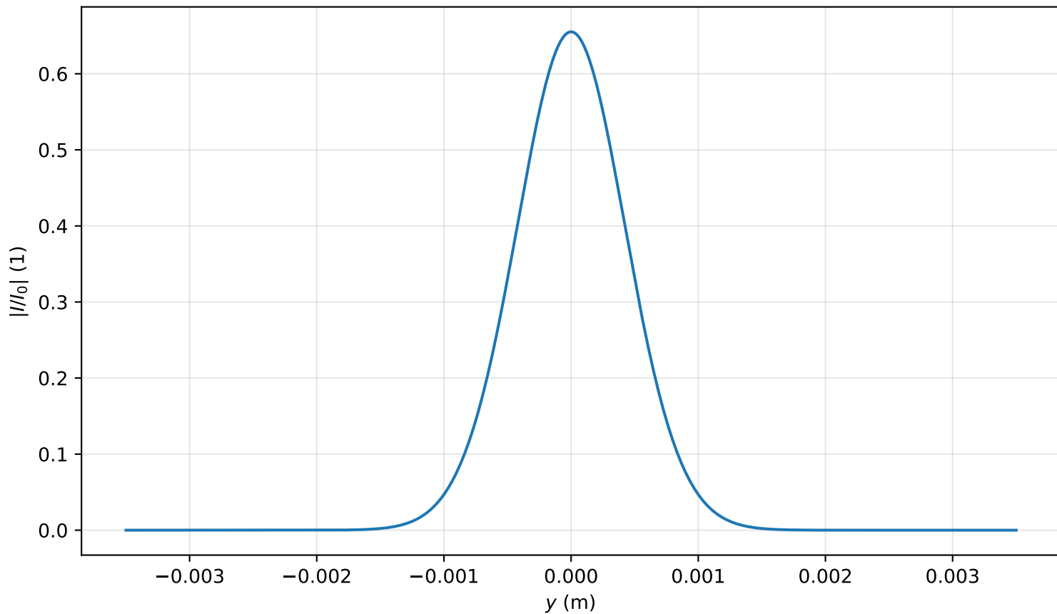
Intensity profile I(x=0, y, z=1.592)/I_0 , P_{in}=0.1P_{cr} , artificial time
